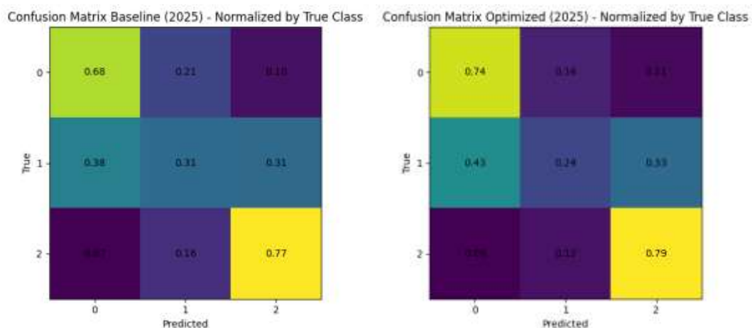
Gambar 7. Confusion matrix model baseline (Kiri) dan confusion matrix model teroptimasi
